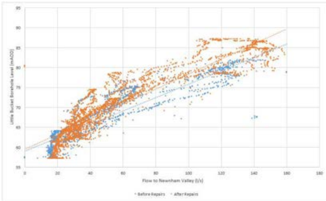
Figure 5.2 – Long Term Monitoring (Dec 2009 to Feb 2021)
