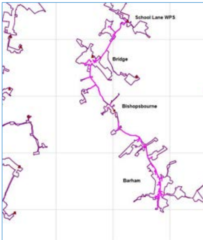
Figure 3.1 sewers electroscan surveyed Barham to Bekebourne (shown in pink), catchment boundary in purple.
