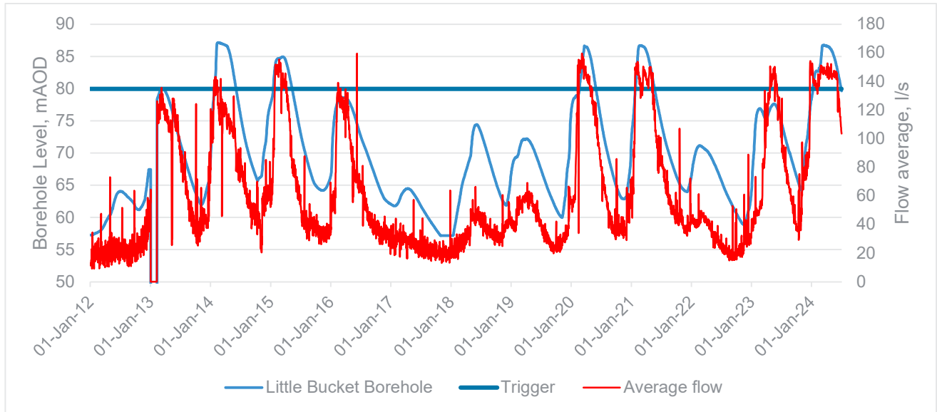
Figure 5.1 – recorded data with trigger levels
