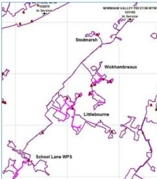
Figure 3.2 sewers electroscan surveyed Bekebourne to Newnham Valley WTW, (shown in pink), catchment boundary in purple.
